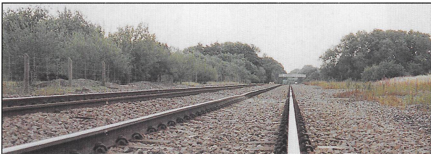
Typical top fault on wet bed site showing a single irregularity
