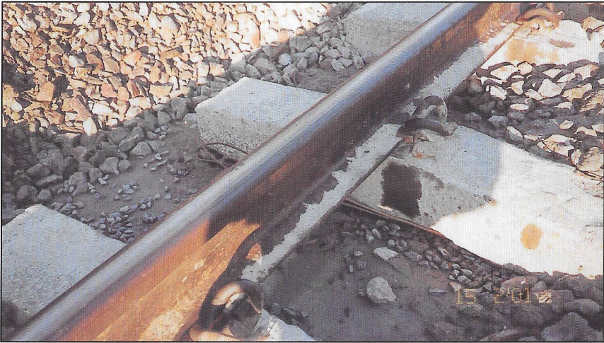
Wet Bed Site: Ballast removed to allow "Drying Out". This causes track distortion or buckling in hot weather
