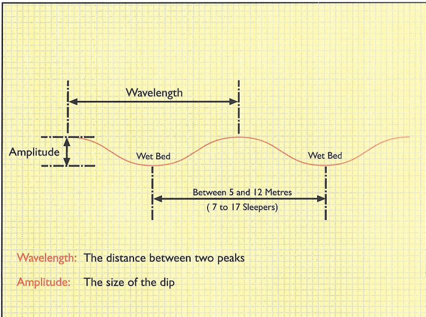
Wavelength and Amplitude of Cyclic Wet Beds
