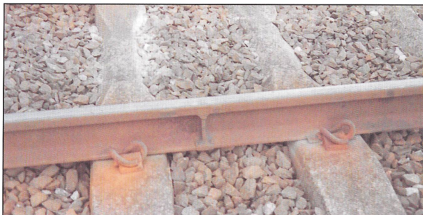
Pads out on a weld. Onset of a wet bed.
