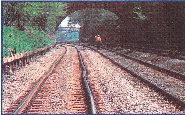
In the picture above we can see the result of hot weather on incorrectly maintained track - in this case poorly installed ballasted steel sleepers.
