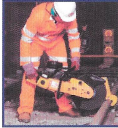
Rail Mounted Disc Saw for cutting rails
