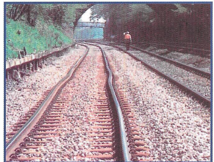
Misalignment provides a trigger point for track buckles
