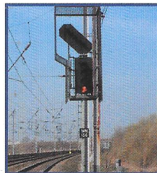
A three aspect signal with route indicator to indicate when trains are to transfer from one line to another
