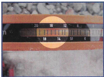
Twist Measurement is Read Off
