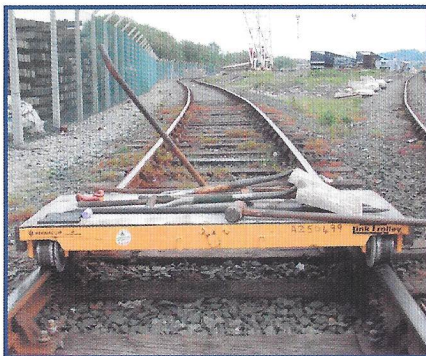
Fig 3.The device shown is known as a rail trolley, is more robust than the rail skate, running on both rails it allows the workers to carry larger items for example sleepers, timbers, large tools, small plant etc (only to be used with the permission of the signaller and under strict controls.)
