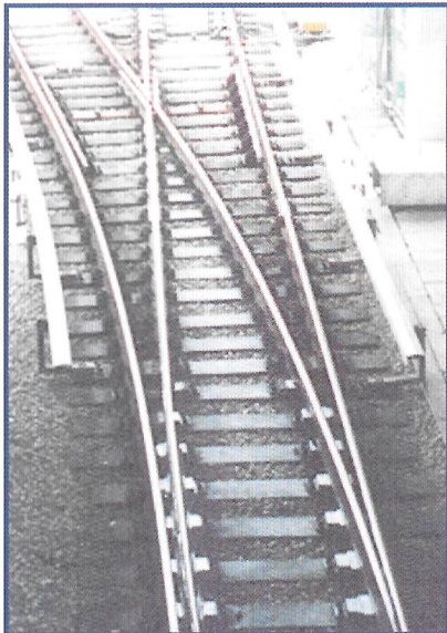
Left Hand Turnout
