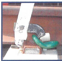
White ePlus Panpuller / Extractor for use with the Pandrol™ ePlus system "pulling in"
