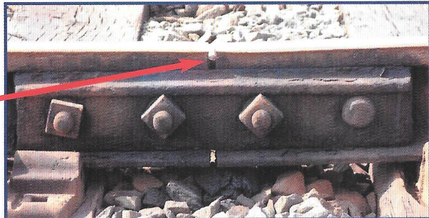
A typical Flat Bottom Fishplate
