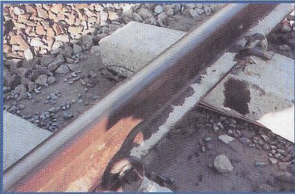
The Wet bed has developed to a point where if the ballast was removed it could result in buckling/distortion of the track.
