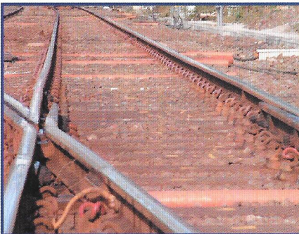
Less severe misalignment on left hand rail just off the crossing nose
