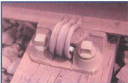
Mills Rail Clip
