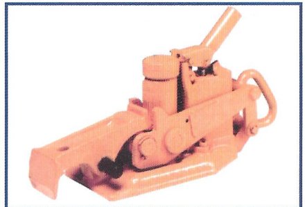
Stumec Hydraulic Track Aligner For Aligning /Slewing and Lifting Track Can be Used Under Traffic
