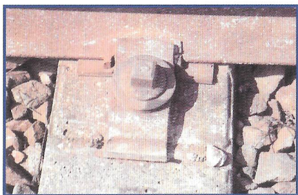
RD Fastening
