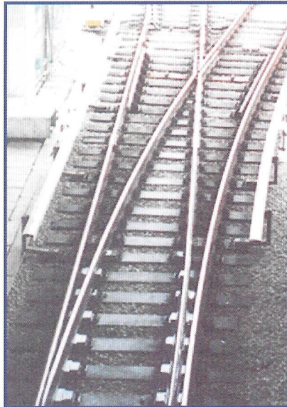
Right Hand Turnout
