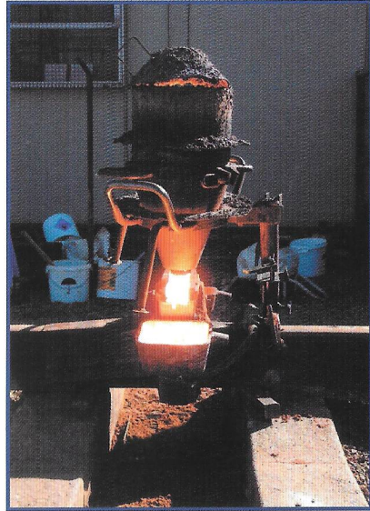
Stage 2 The crucible mixture is ignited. When the molten metal reaches the required temperature it is poured into the mould.
