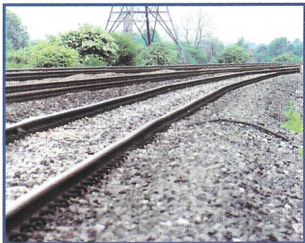
Poor Top In Continuous Welded Rail(CWR) On Concrete Sleepers
