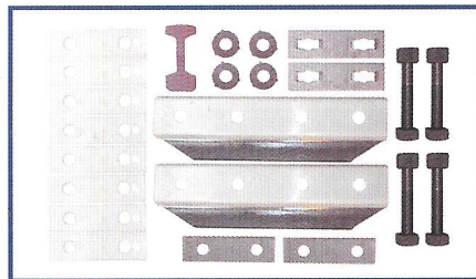
Insulated 4 hole skirted fishplate Assembly for Bull Head rail joint
