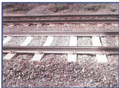
The result of neglected drainage, advanced stages of ballast attrition.
