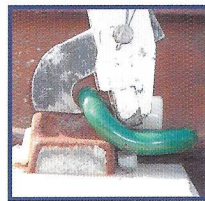
White ePlus Panpuller / Extractor for use with the Pandrol™ ePlus system "extracting"
