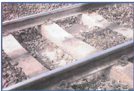
The result of neglected drainage, advanced stages of ballast attrition.
