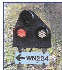
A ground signal to allow for controlling trains out of sidings on to a main line
