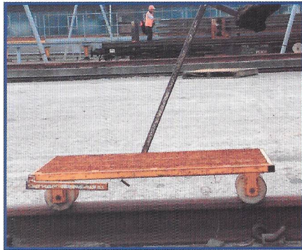
Fig 2. Shows a device that can be positioned on one rail to enable small heavy items such as fishplates, bags of chippings, bags of bolts etc to be pushed to the site of work by one person. (maximum weight permitted 25kg)
