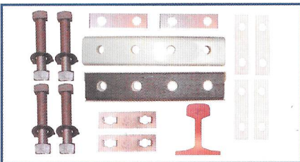
Burns Flat Bottom 4 Hole Insulated Joint Assembly
