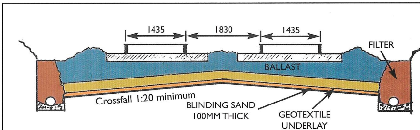
SAND BLANKET - TYPICAL CROSS SECTION FOR STRAIGHT TRACK
