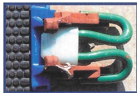
Pandrol™ Fastclip Assembly
