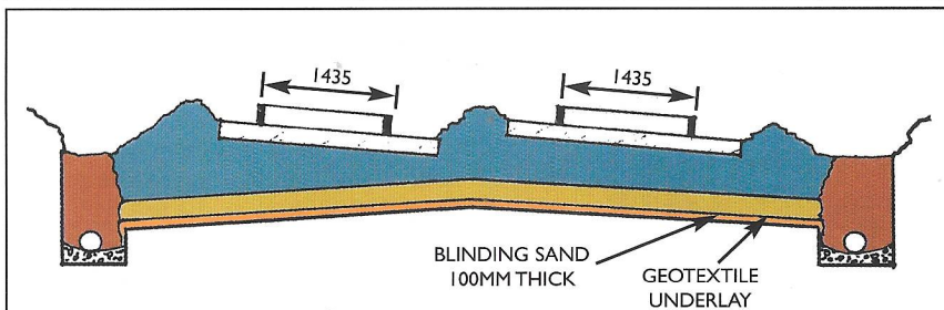
SAND BLANKET - TYPICAL CROSS SECTION FOR CURVED TRACK
