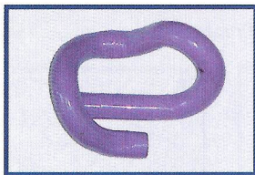
Pandrol™ PR427A Clip. (maintenance replacement for obsolete PR303)
