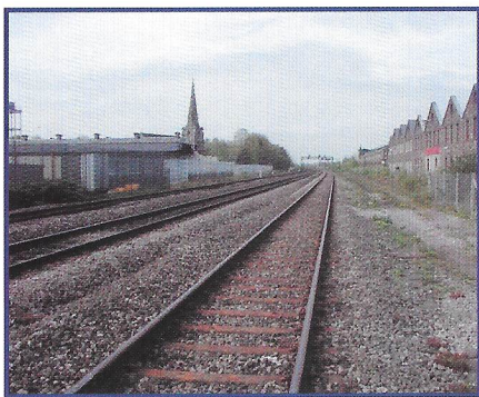
Three Track Situation Consisting of Up Line and Down Line also Bi-Directional Line, allowing trains to travel in both directions over the same portion of line
