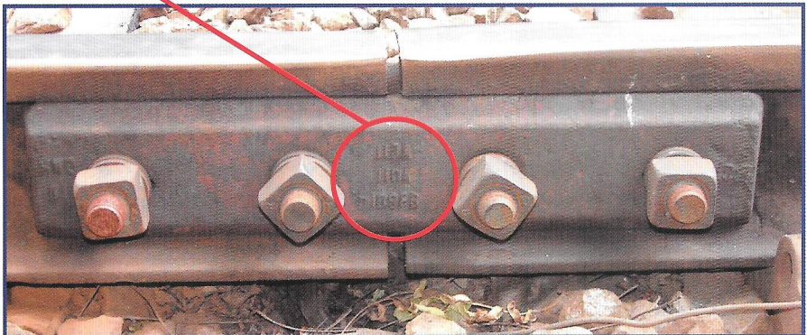
109lb Plate Flat Bottom Rail Pear Shaped Hole
