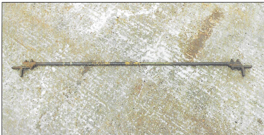
Fig.4. Gauge-setting bar NOT a track gauge
