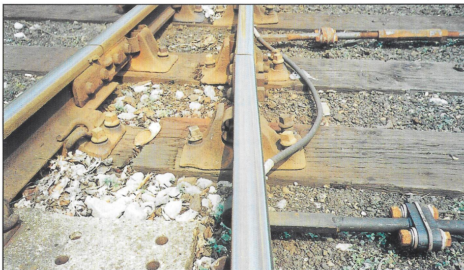
Figure 12 Leaning chairscrews in this S&C indicate gauge spread
